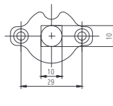
Vierkantlager 10x10mm ID 556
